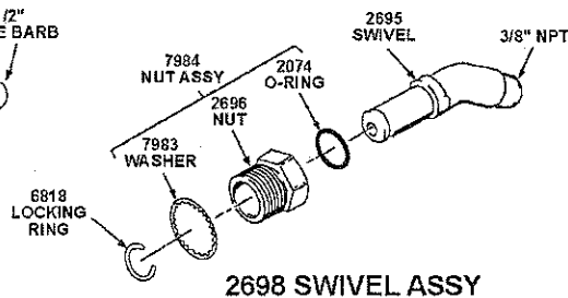
2698 SWIVEL ASSY
