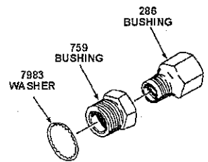
REDUCING BUSHING
