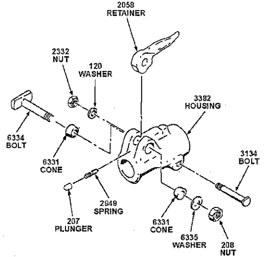
3383 LATCH-TYPE IMPORTANT
