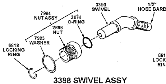
3388 SWIVEL ASSY
