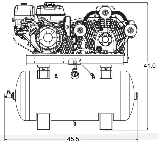
30 GALLON TANK VERSION
