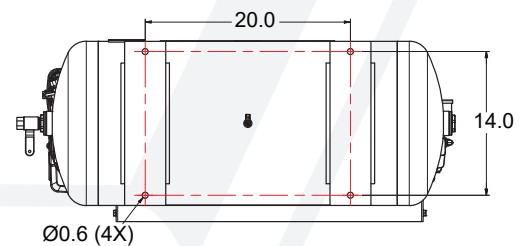
30 GALLON MOUNTING PATTERN
