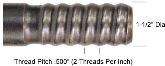
Thread Pitch .500" (2 Threads Per Inch)
